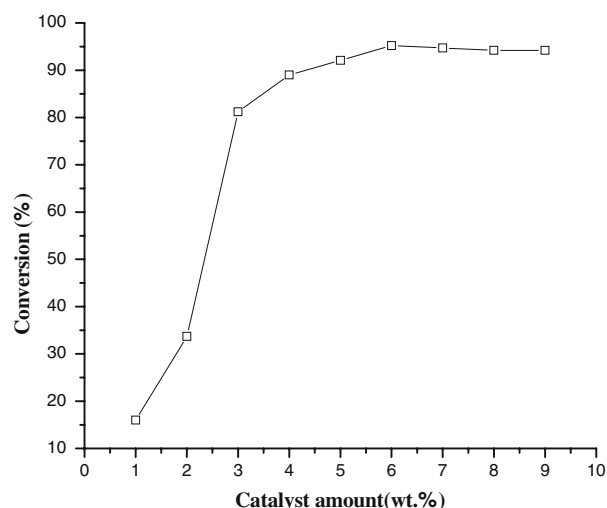
Figure 5. Conversions of soybean oil as a function of catalyst amount. Reaction conditions: methanol/oil molar ratio 12:1, reaction time 1 h, reaction temperature 338 K.
