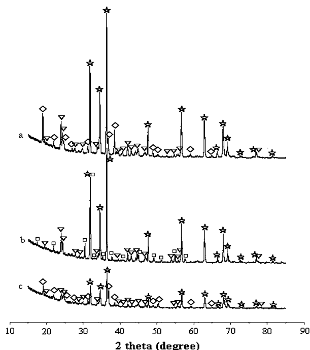
Figure 1. XRD patterns for samples: (a) 2.5 mmol/g Ba–ZnO calcined at 873 K, (b) 2.5 mmol/g Ba–ZnO calcined at 1073 K and (c) 4 mmol/g Ba–ZnO calcined at 873 K. (☆), ZnO; (▽), \text{BaCO}_3 ; (◇), \text{Ba}(\text{NO}_3)_2 ; (□), \text{BaZnO}_2 .
